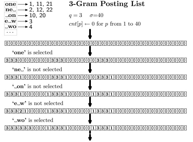
Figure 2: Algorithm Sample
